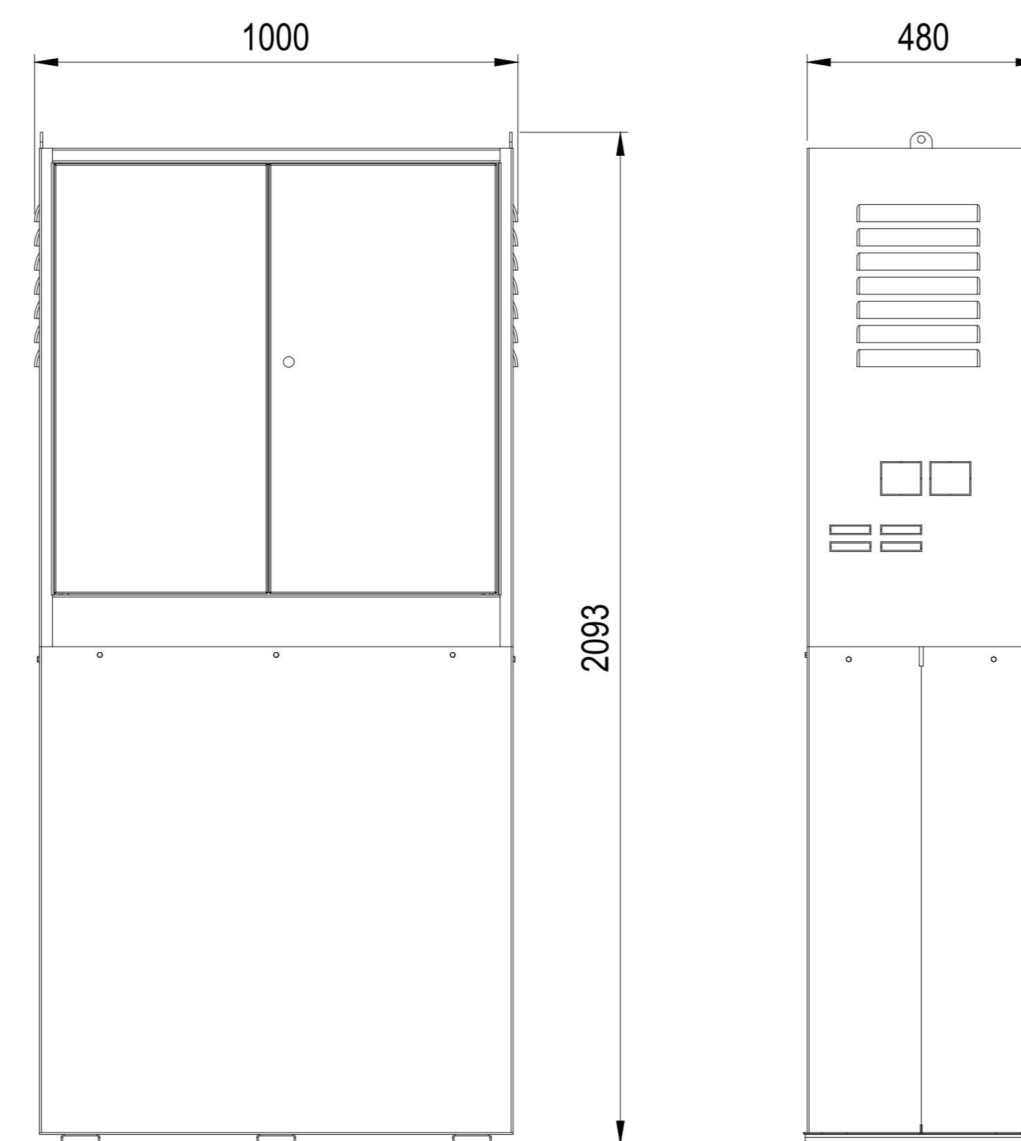
Lift Machinery Cabinet with integrated hydraulic tank. Must be located within 8m of lift well
